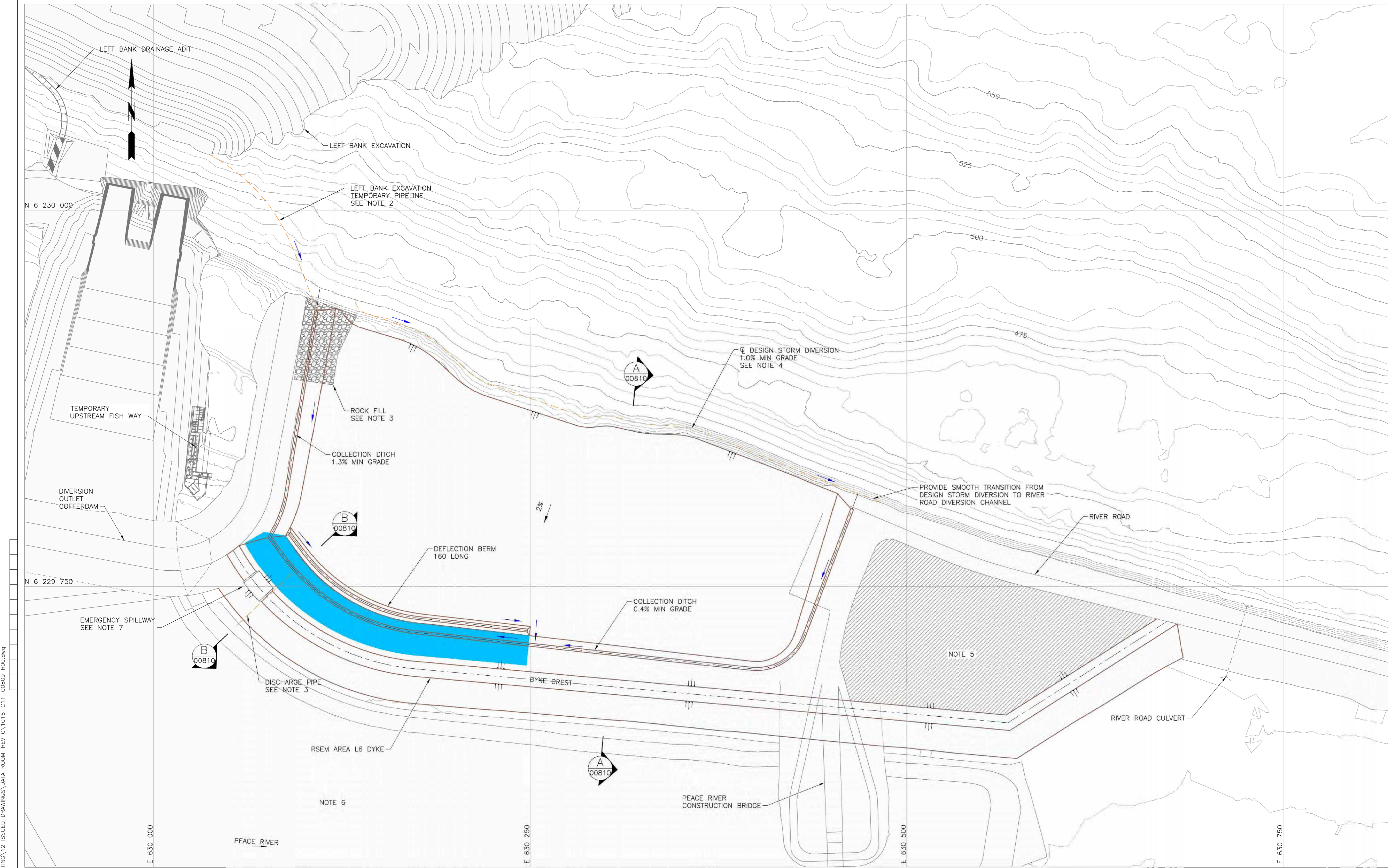
PLAN 1:1000
