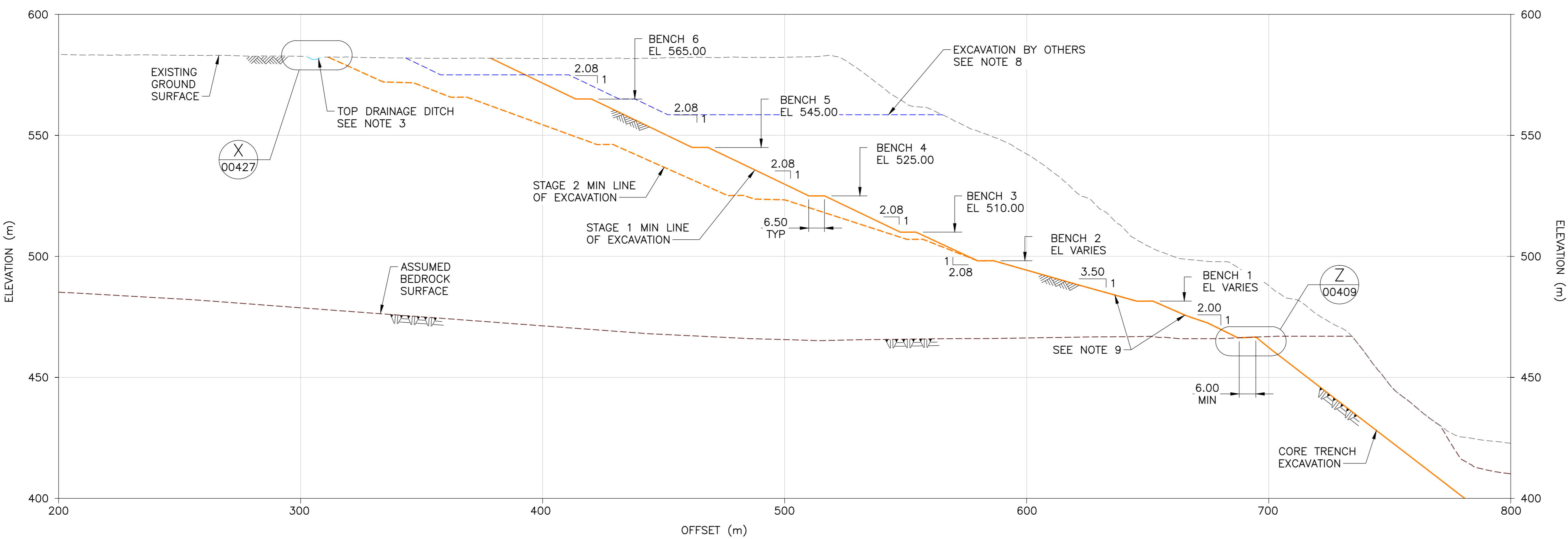
SECTION 1:1000
