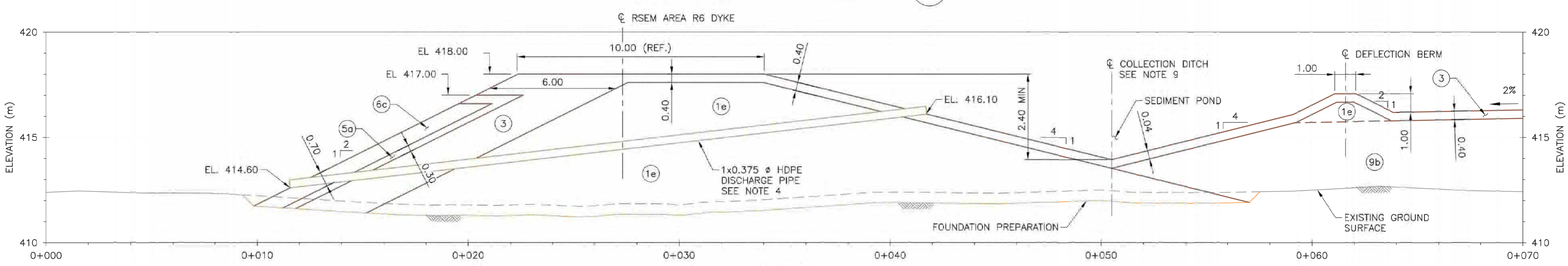
SECTION B 1:100
