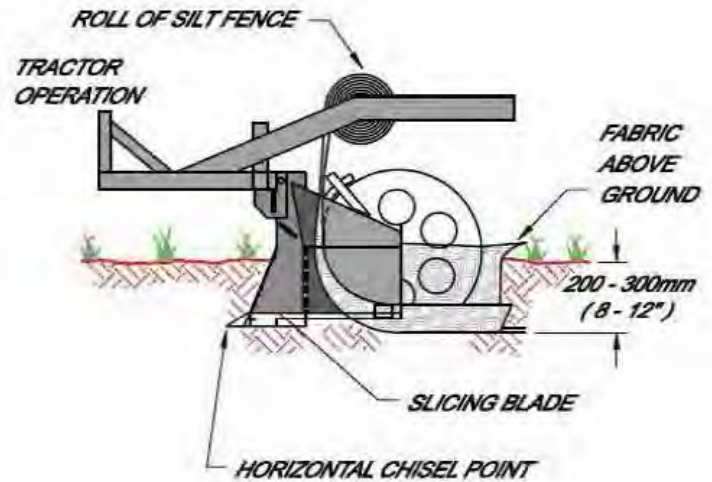
STATIC SLICING METHOD SIDE VIEW
