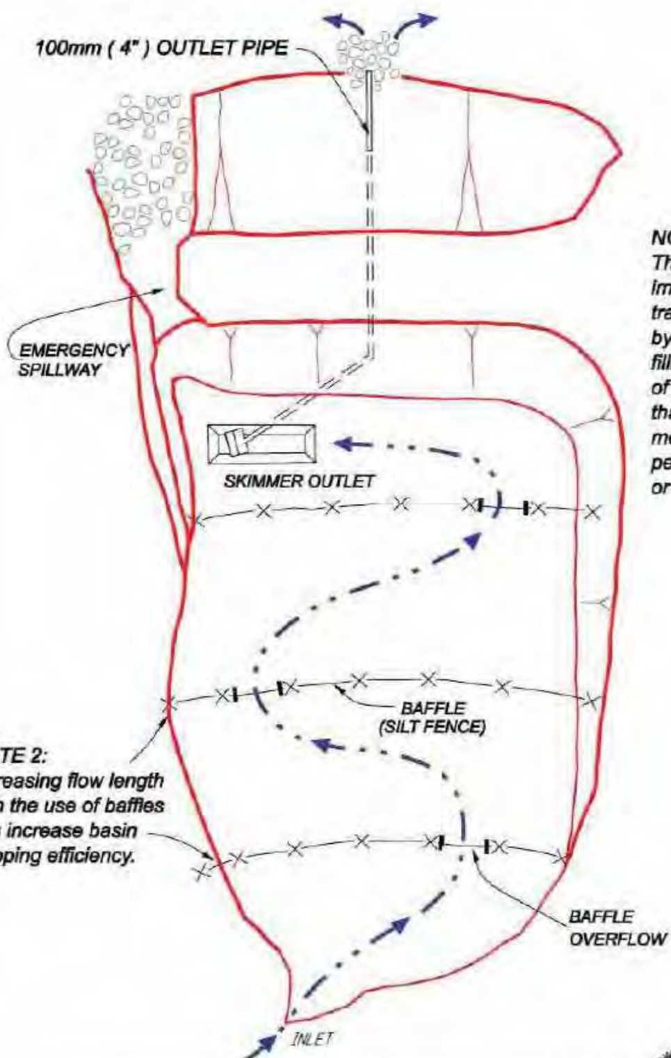
Sediment Basin with Baffles and Skimmer Outlet
