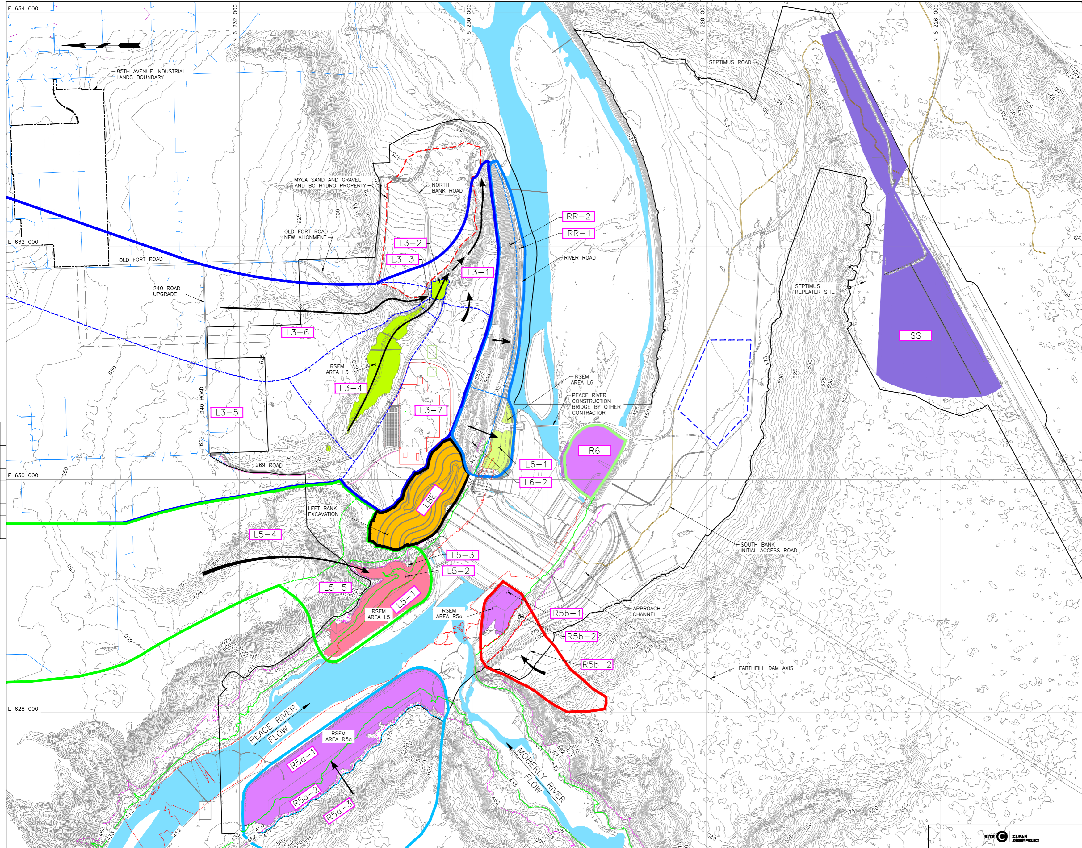
PLAN 1:10000
