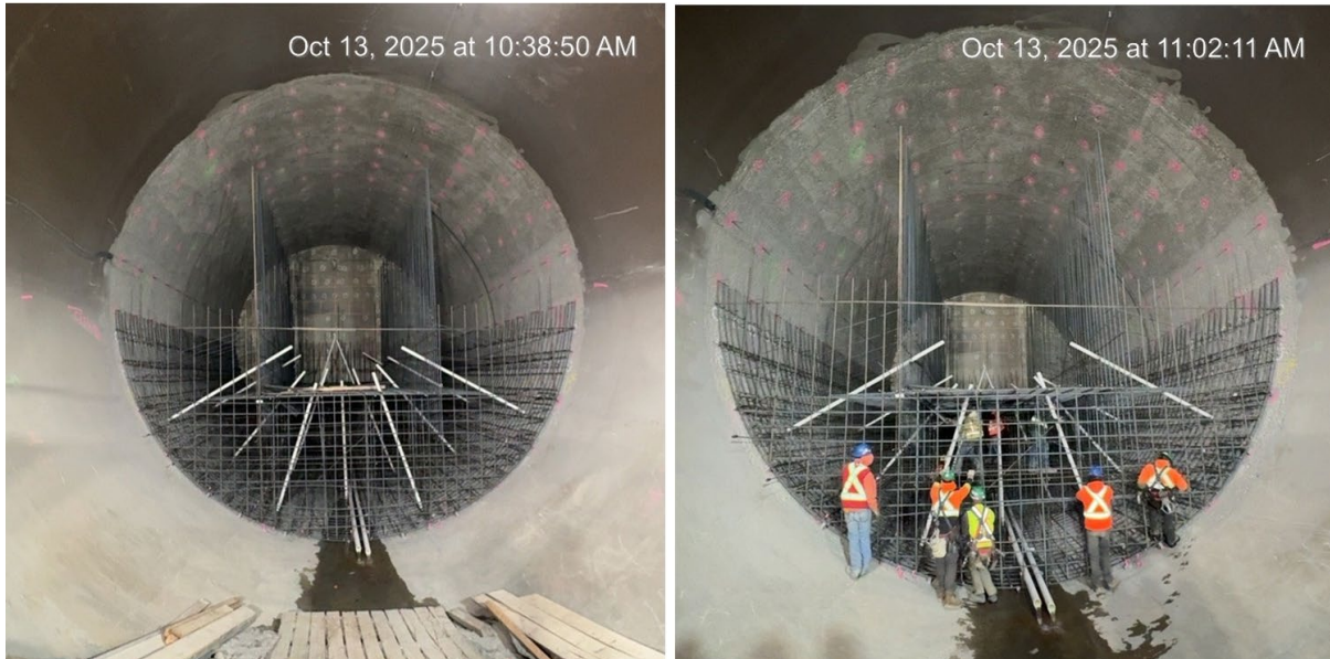
Figure A-7 Construction of the concrete plug for the Diversion Tunnel 1 backfilling. Carpenters are installing formwork coil rods and crews are completing rebar installation. (October 2025)
