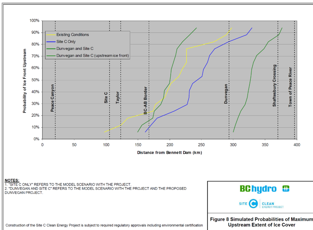
Figure3-7: Simulated probabilities of maximum upstream extent of the ice cover based on simulated winters 1995-1996 to 2010-2011 for without Site C (yellow line) and with Site C (blue line). Green lines for Dunvegan Project can be ignored as this is no longer a viable project Source: Site C EIS Appendix G, Section 4.1, Figure 8.
