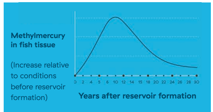
Methylmercury in fish tissue.
